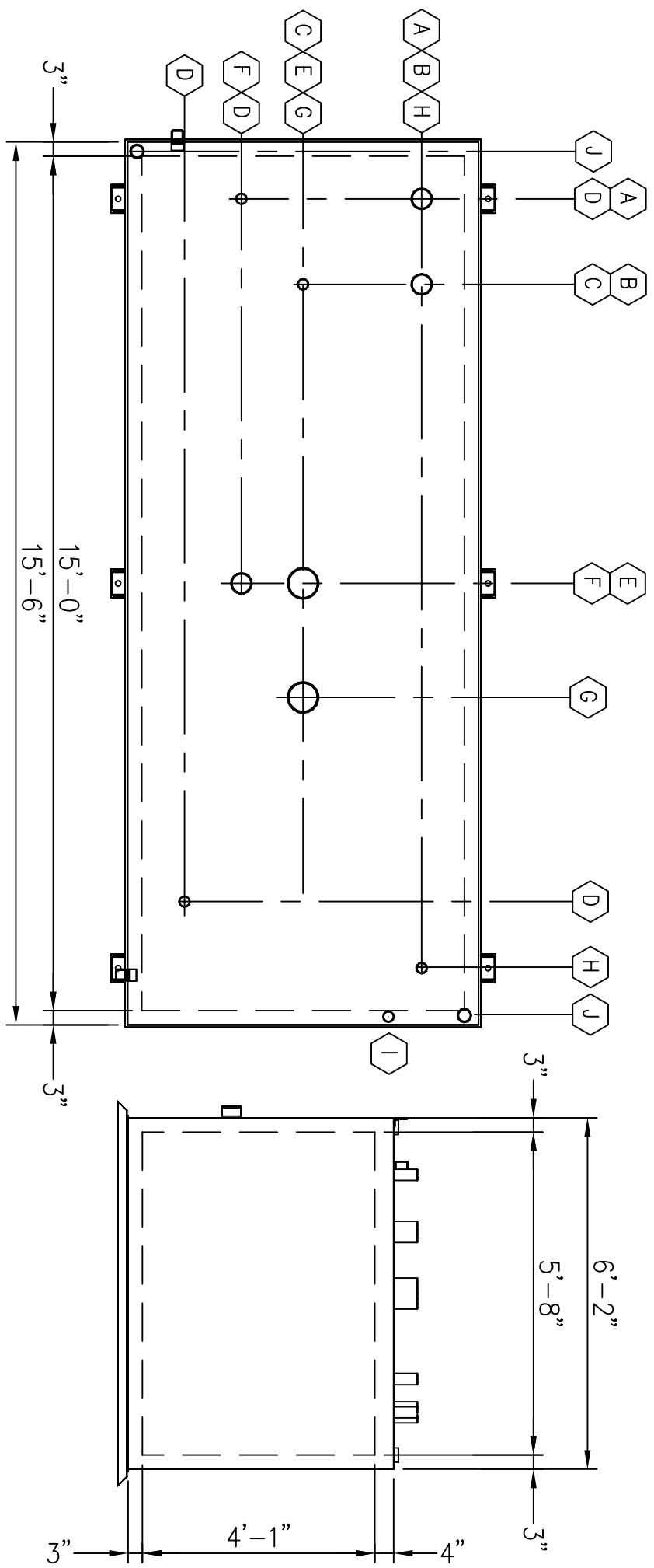
PLAN VIEW
